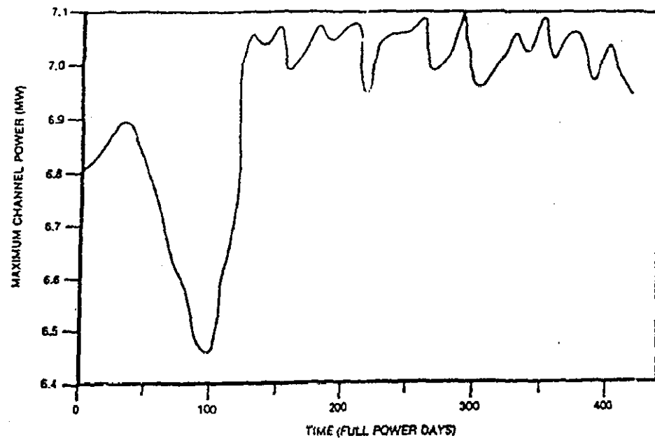
Figure 8-2: Maximum Channel Power.
