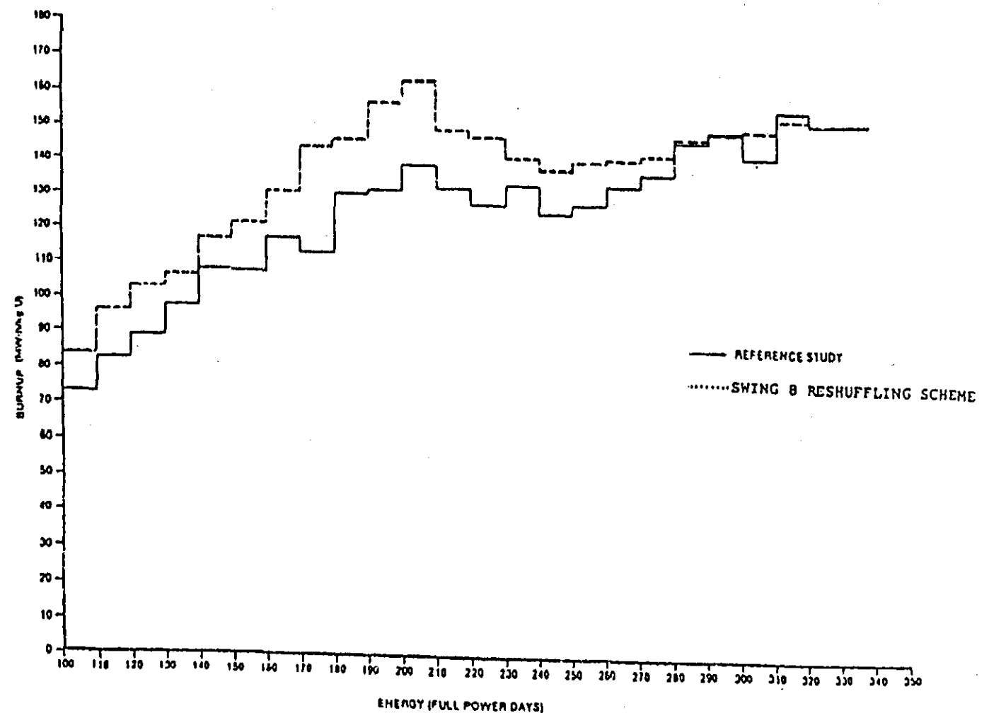
Figure 8-9: Average Discharge Burnup per 10 FPD Interval.
